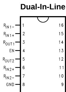
Figure 1. See Package Number D (R-PDSO-G16)
