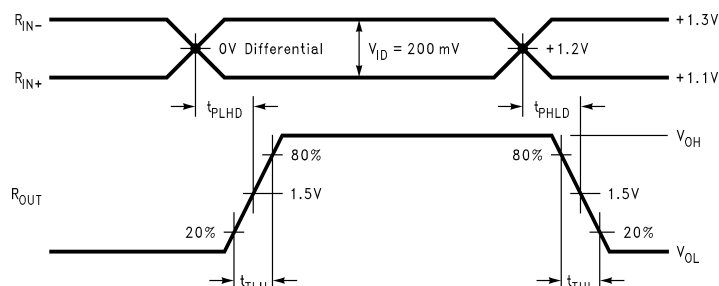
Figure 4. Receiver Propagation Delay and Transition Time Waveforms
