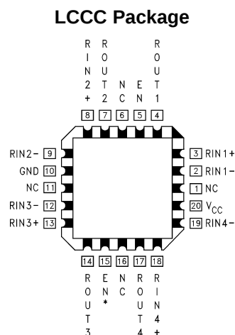
Figure 2. See Package Number NAJ0020A For complete Military Specifications, refer to appropriate SMD or MDS
