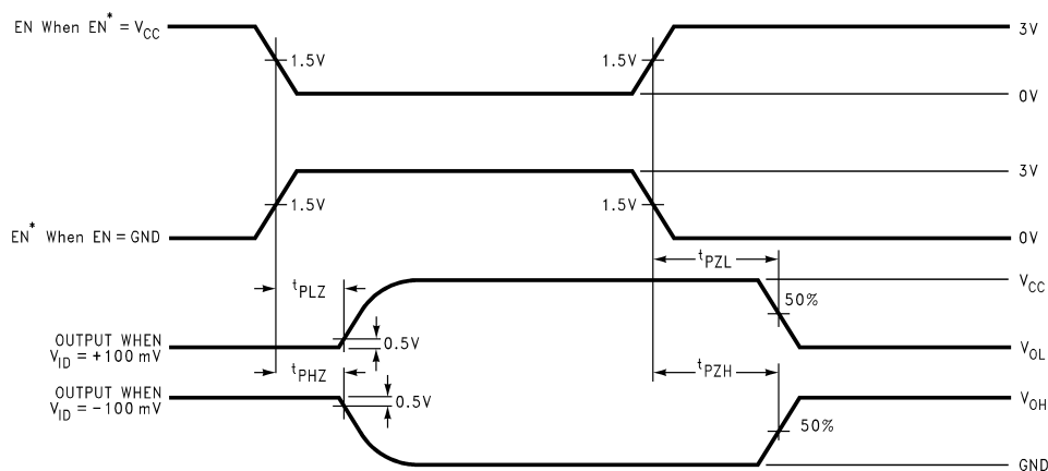
Figure 6. Receiver TRI-STATE Delay Waveforms
