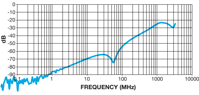
Preliminary AVX W3F41A1018AT Typical Far-side XTALK Elements 2 - 3
