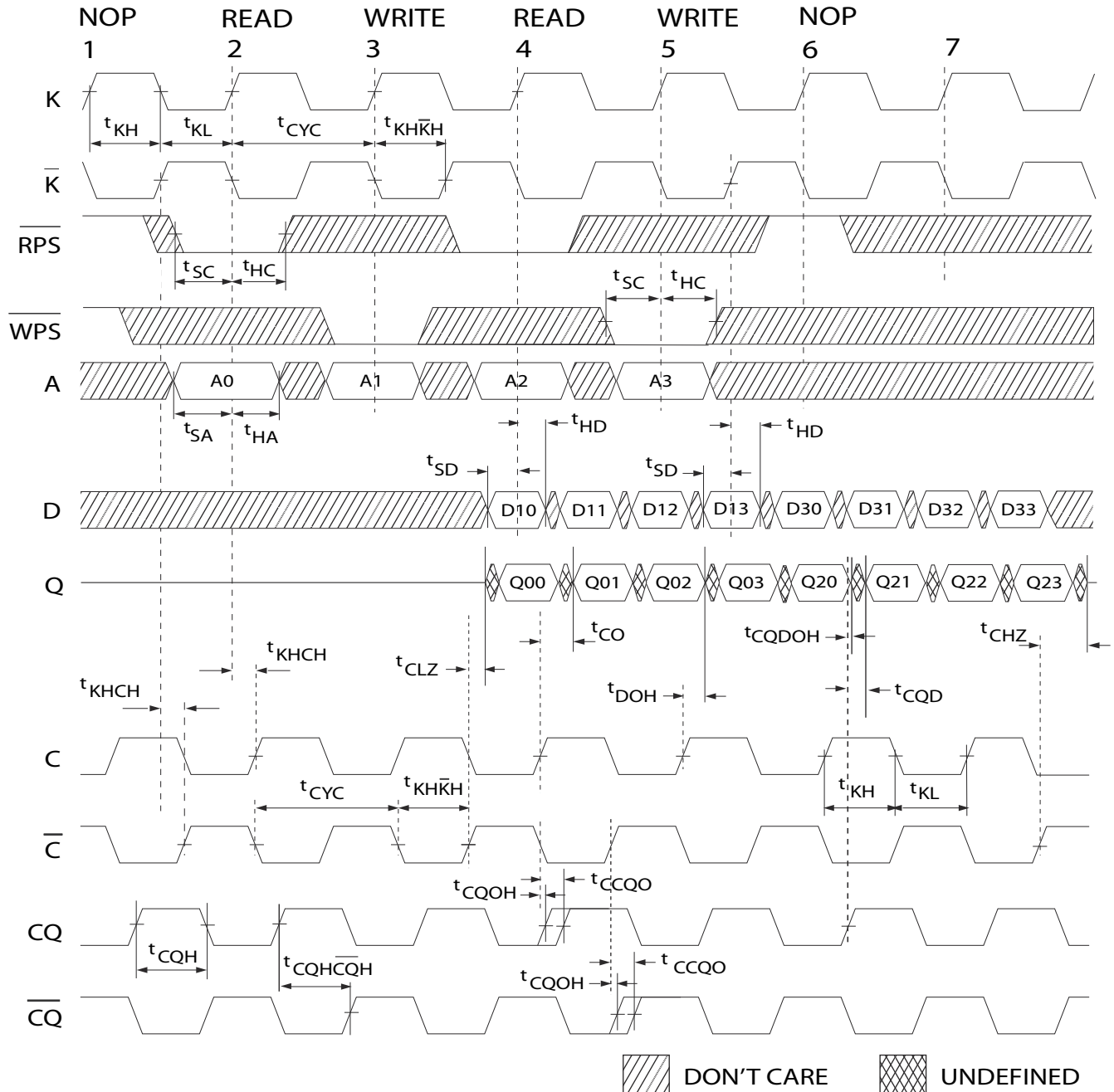
Figure 6. Read/Write/Deselect Sequence [38, 39, 40]
