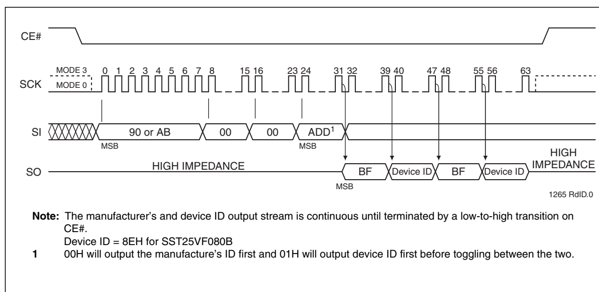
Figure 21: Read-ID Sequence
