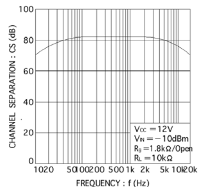
Fig.6 Channel separation
