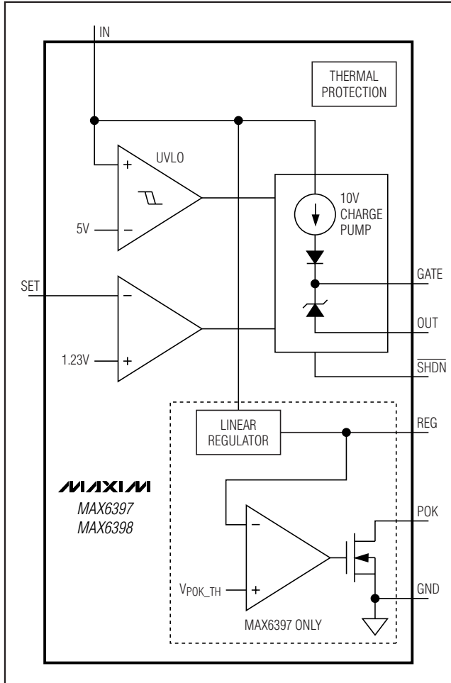
Figure 1. Functional Diagram
