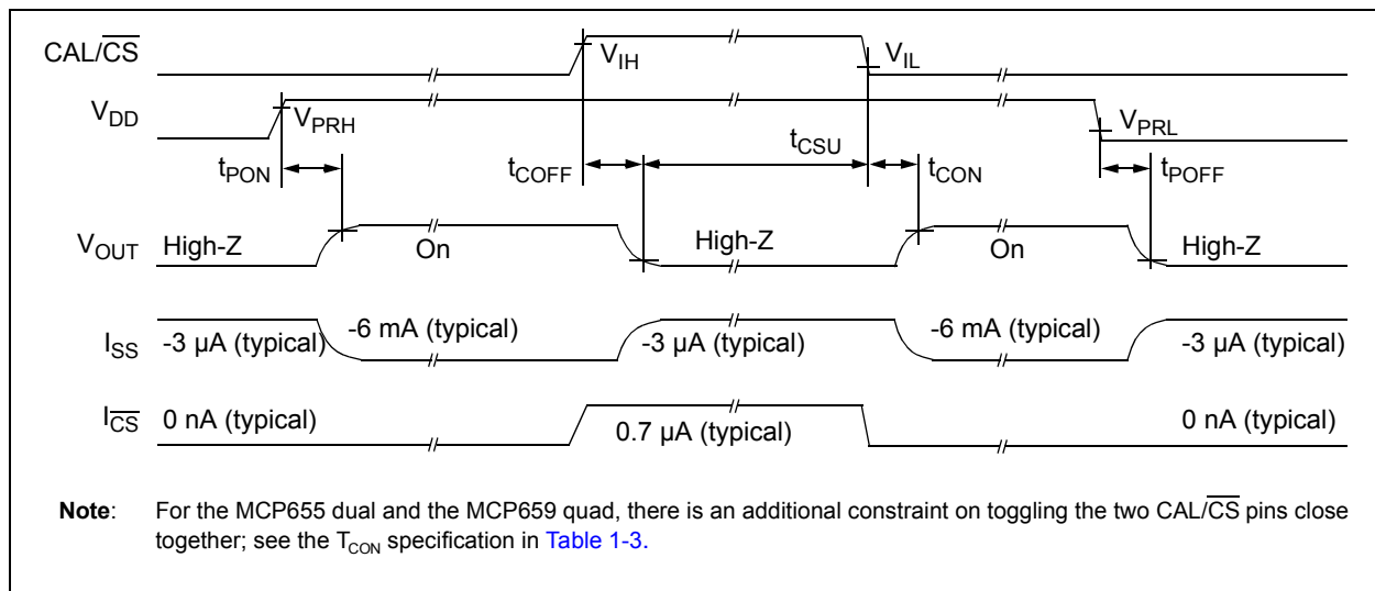
FIGURE 1-1: Timing Diagram.
