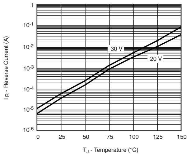
Reverse Current
