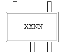
5-Lead SC70 (MCP6401 only)
