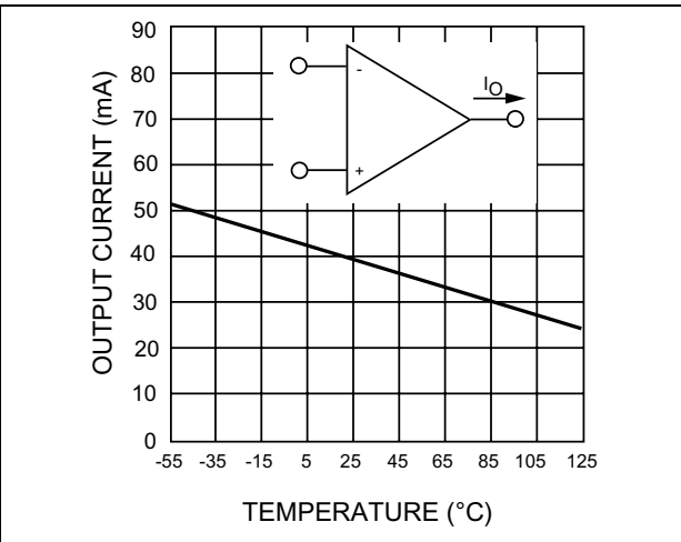
Figure 4. Current limiting
