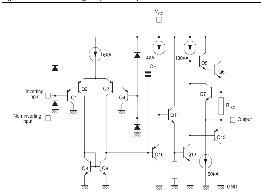
Figure 1. Schematic diagram (1/4 LM2902)
