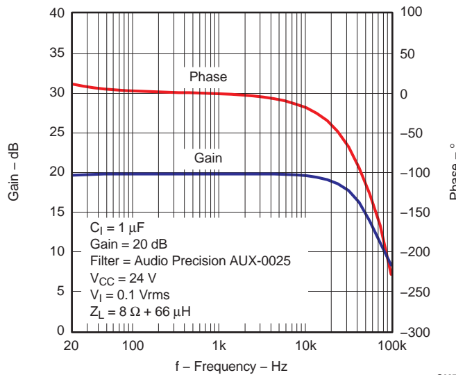
GAIN/PHASE vs FREQUENCY (PBTL)
