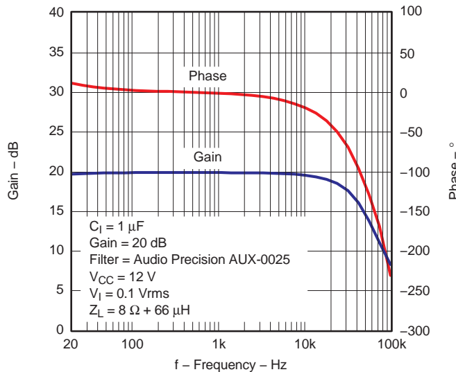
GAIN/PHASE vs FREQUENCY (BTL)
