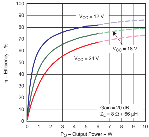
EFFICIENCY vs OUTPUT POWER (BTL)
