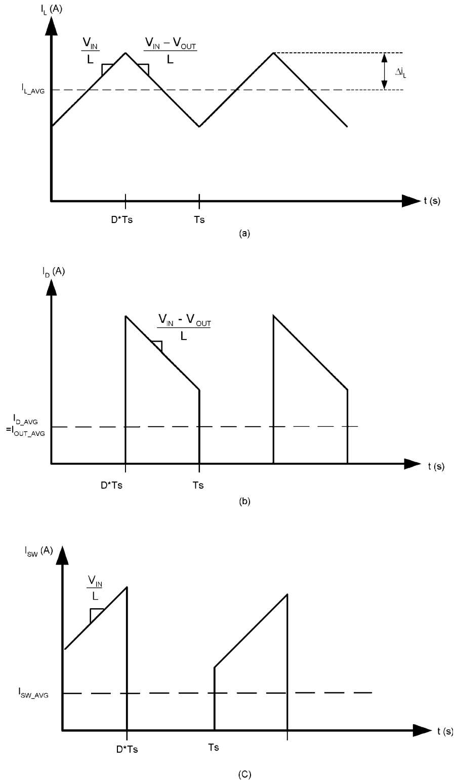
FIGURE 12. A. Inductor Current B. Diode Current
