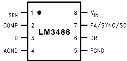
8 Lead Mini SO8 Package (MSOP-8 Package) 10138802
