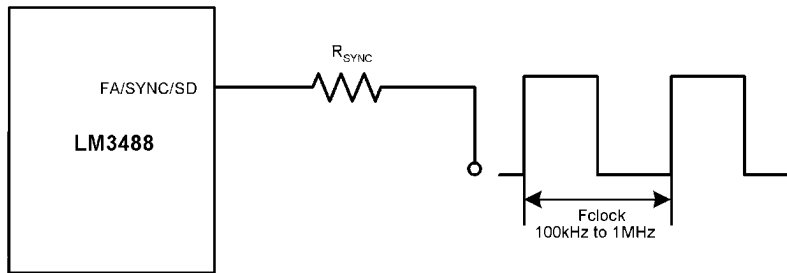
FIGURE 7. Frequency Synchronization
