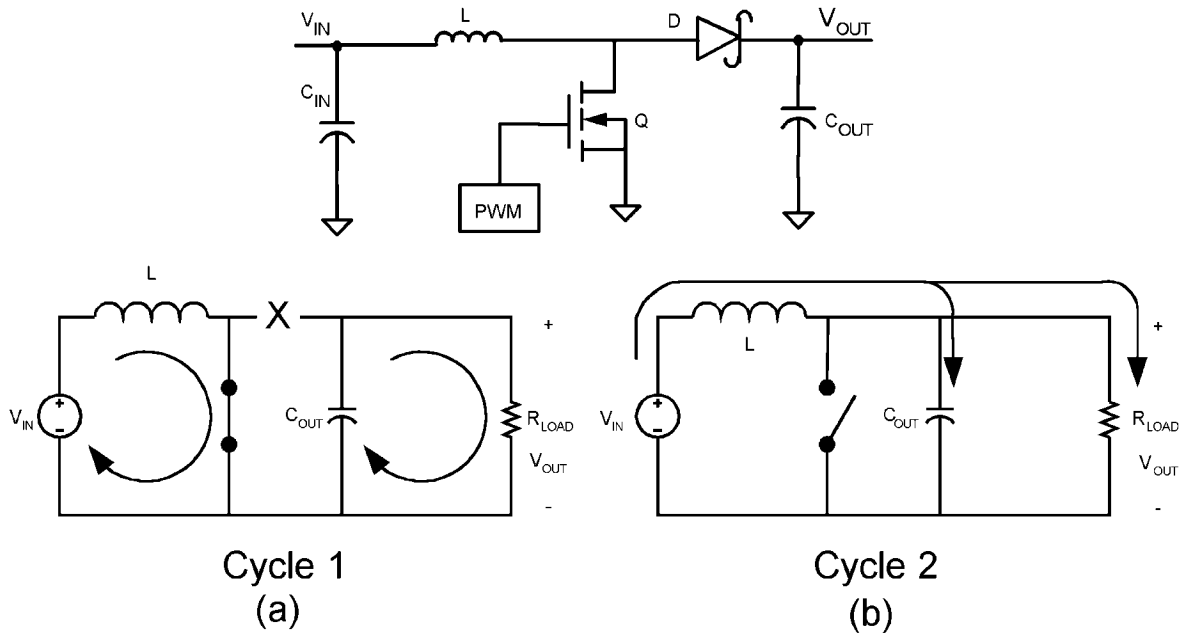
FIGURE 11. Simplified Boost Converter Diagram (a) First cycle of operation. (b) Second cycle of operation
