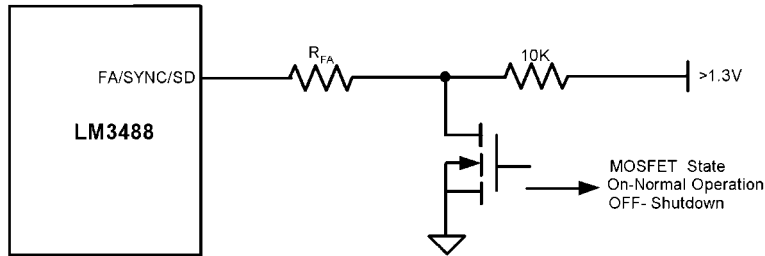
FIGURE 8. Shutdown Operation in Frequency Adjust Mode
