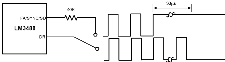
FIGURE 9. Shutdown Operation in Synchronization Mode
