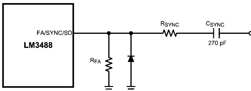
FIGURE 10. Frequency Adjust or Frequency Synchronization
