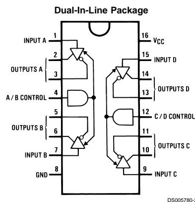
Top View Order Number DS3487M or DS3487N See NS Package Number M16A or N16E
