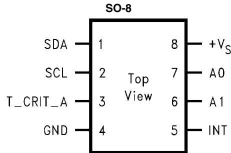
LM76 See NS Package Number M08A
