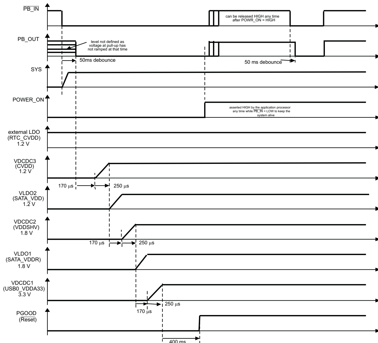
Figure 50. Timing for OMAP-L138
