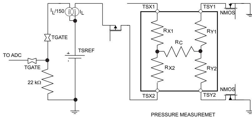
Figure 36. Pressure Measurement
