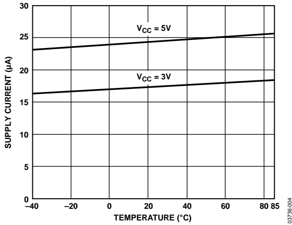
Figure 4. Supply Current vs. Temperature (No Load)
