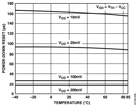
Figure 6. Power-Down RESET Delay vs. Temperature ADM8_T/S/R/Z
