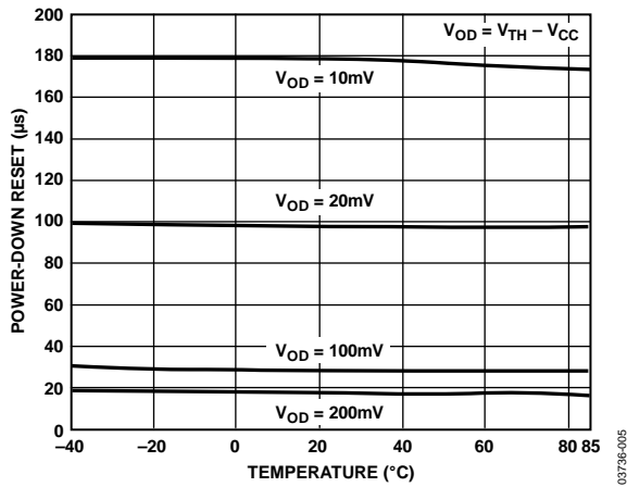
Figure 5. Power-Down RESET Delay vs. Temperature. ADM8_L/M/J
