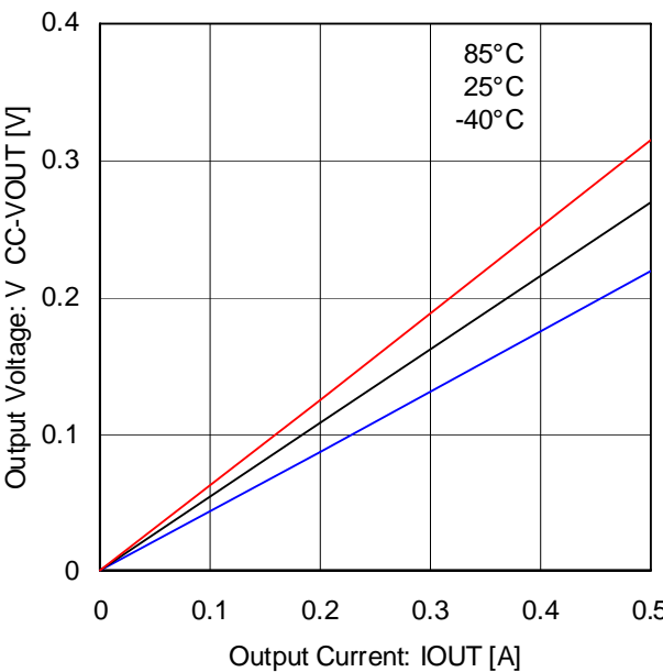
Fig.18 Output high voltage (BD6210)
