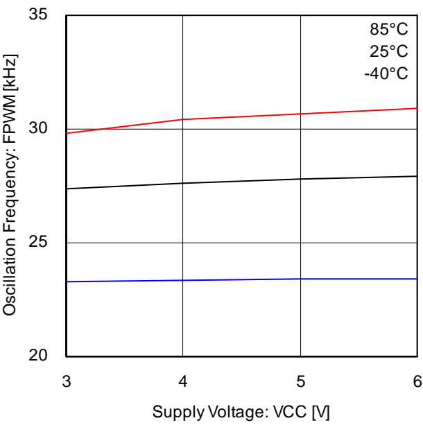
Fig.12 VCC - Carrier frequency
