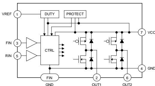
Fig.3 BD6210HFP / BD6211HFP / BD6212HFP
