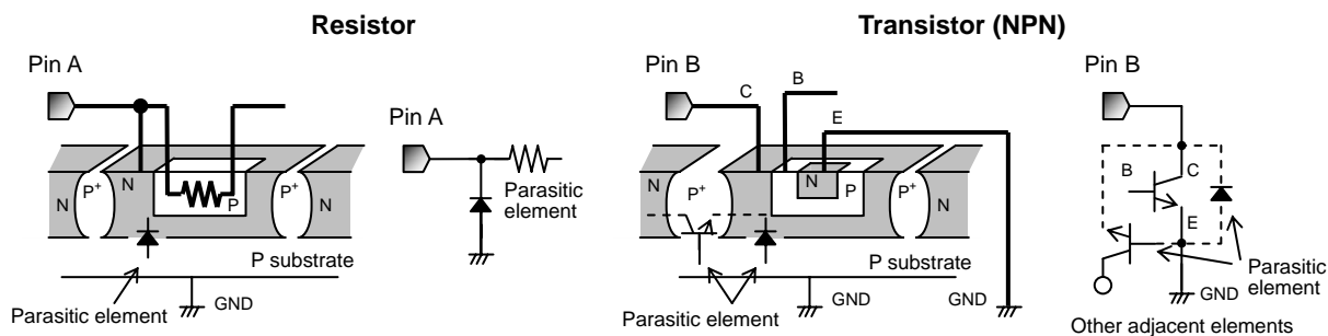
Fig.41 Example of monolithic IC structure
