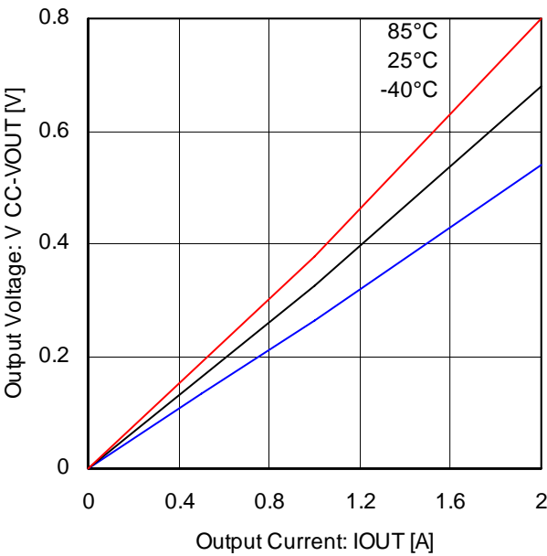
Fig.20 Output high voltage(BD6212)
