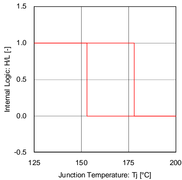
Fig.15 Thermal shutdown
