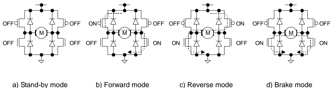
Fig.30 Four basic operations (output stage)
