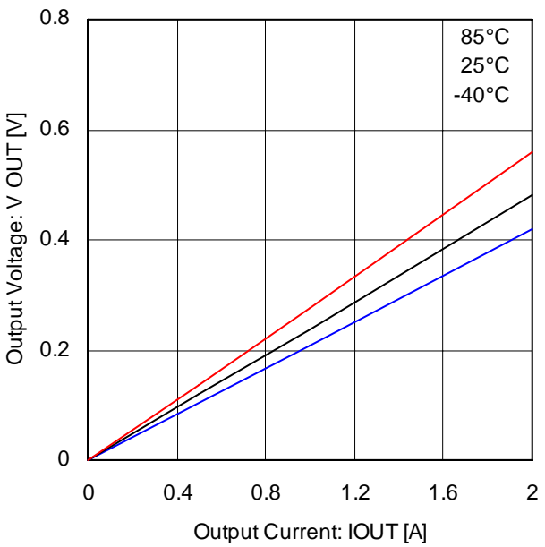
Fig.26 Output low voltage (BD6212)
