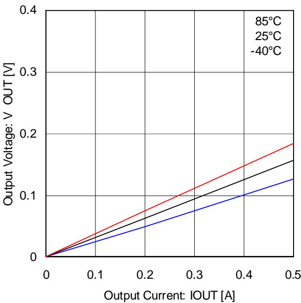
Fig.24 Output low voltage (BD6210)
