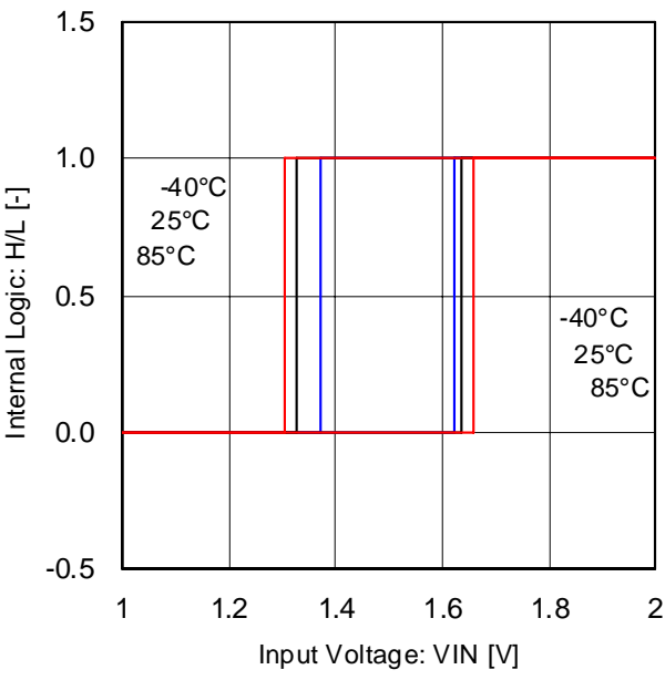
Fig.8 Input threshold voltage
