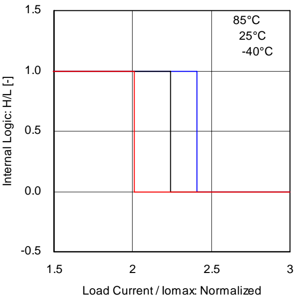
Fig.16 Over current protection (H side)
