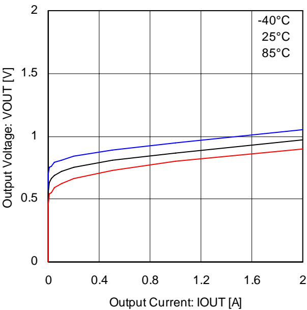
Fig.32 Low side body diode (BD6222)
