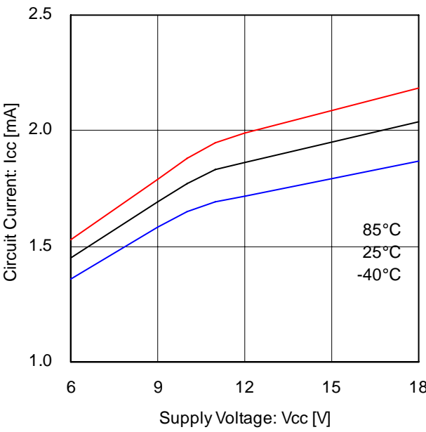
Fig.10 Supply current (2ch)
