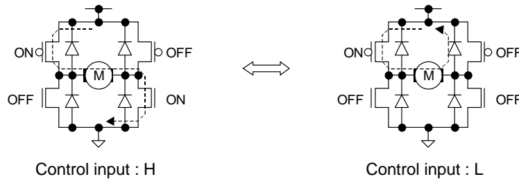
Fig.34 PWM control mode A operation (output stage)
