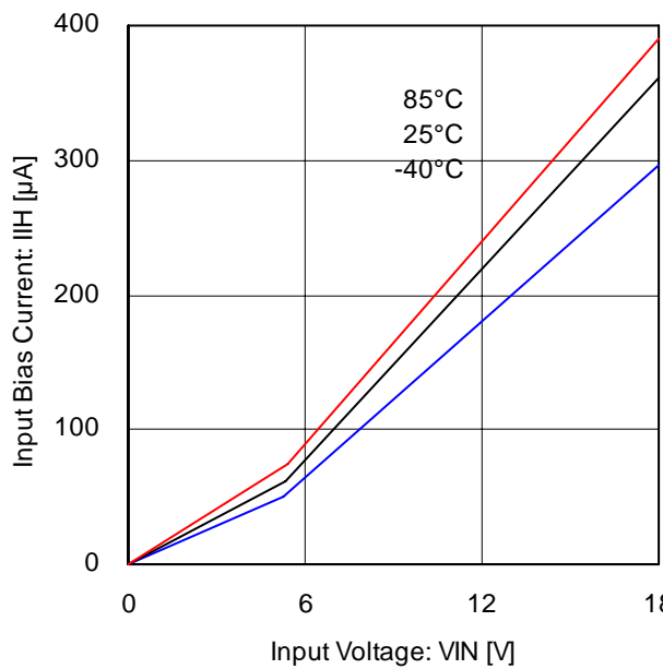
Fig.12 Input bias current
