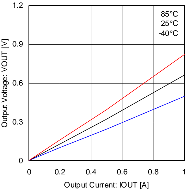
Fig.28 Output low voltage (BD6221/26)
