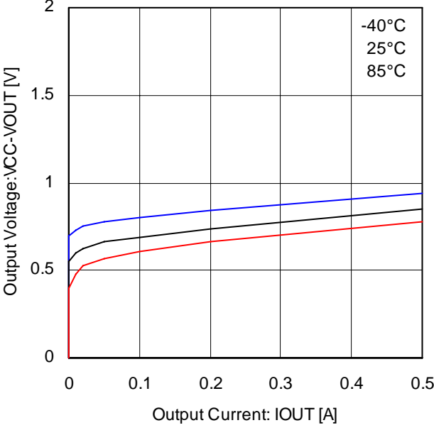
Fig.24 High side body diode (BD6220/25)
