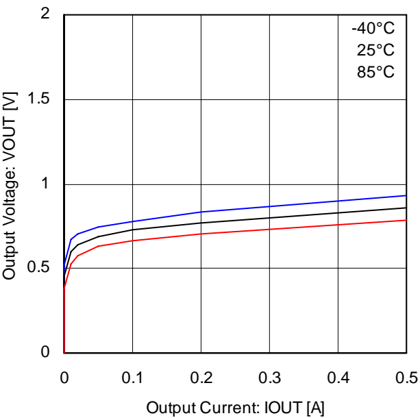
Fig.30 Low side body diode (BD6220/25)
