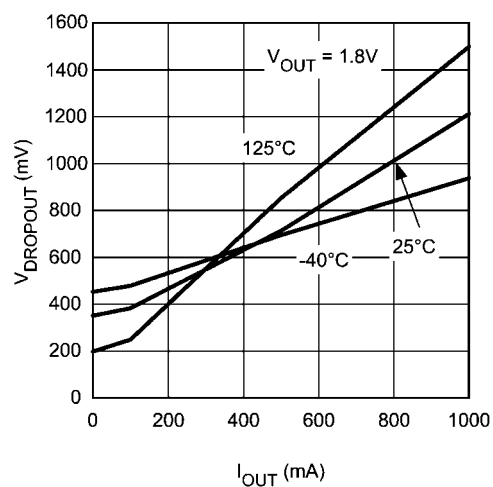
Dropout Voltage vs I_{OUT}
