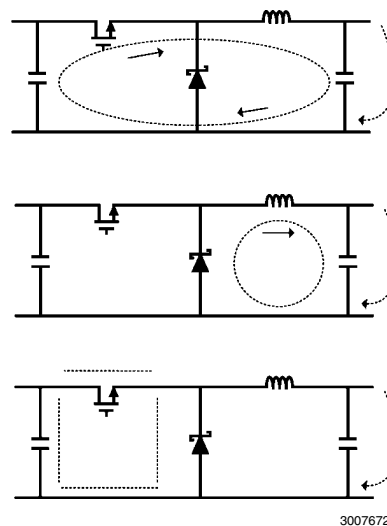
FIGURE 6. Current Flow in a Buck Application
