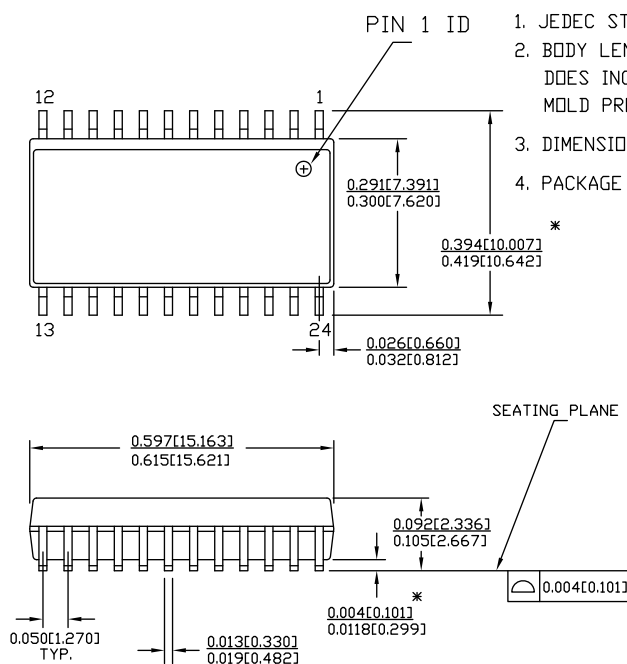
Figure 53. 24-pin SOIC (0.615 x 0.300 x 0.0932 Inches)
