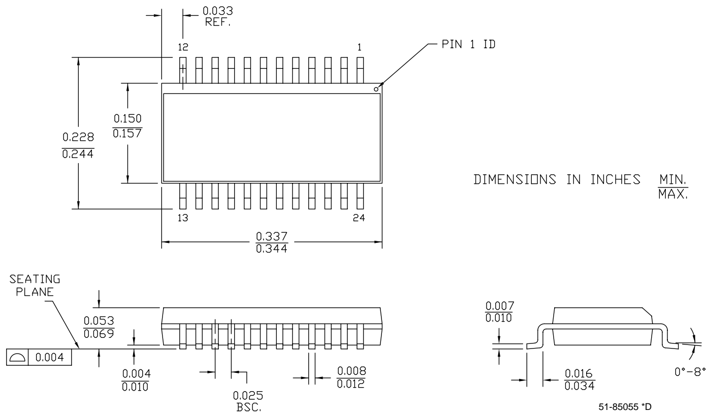
Figure 55. 24-pin QSOP (8.65 × 3.9 × 1.44 mm)
