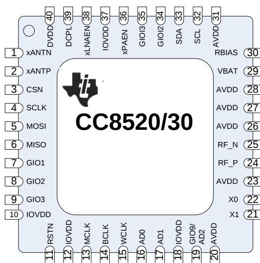
Figure 1 - CC8520/CC8530 QFN Package Top View
