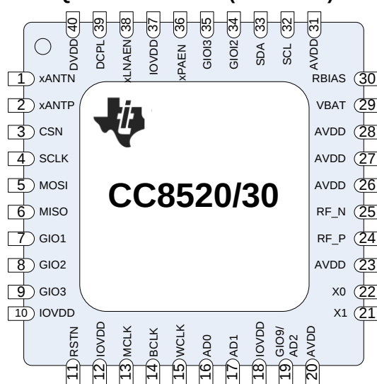
QFN-40 PACKAGE (TOP VIEW)
