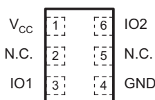
DRY PACKAGE (TOP VIEW)
