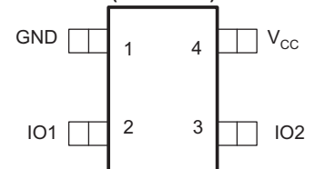
DZD PACKAGE (TOP VIEW)
