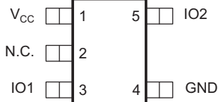
DRL PACKAGE (TOP VIEW)
