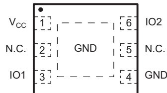
DRS PACKAGE (TOP VIEW)
