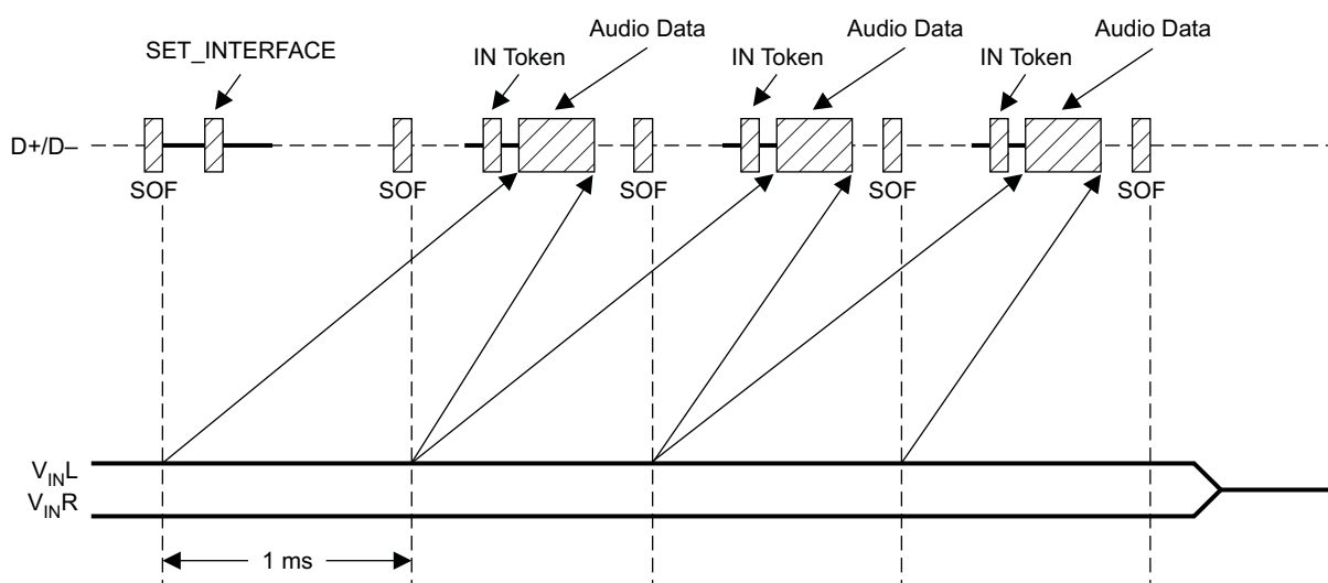
Figure 34. Record Sequence
