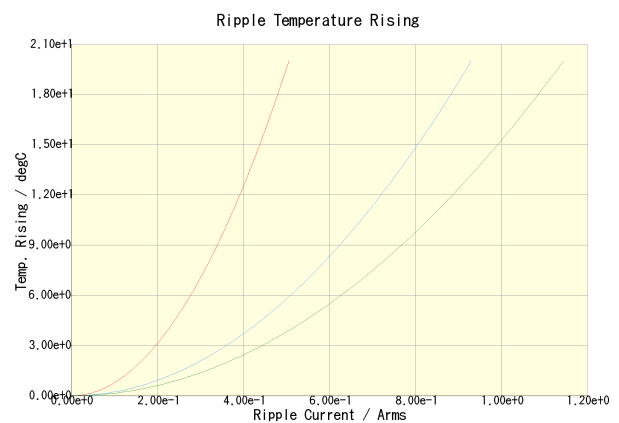
C1608X7R1C224K080AC(100kHz) C1608X7R1C224K080AC(500kHz) C1608X7R1C224K080AC(1MHz)
