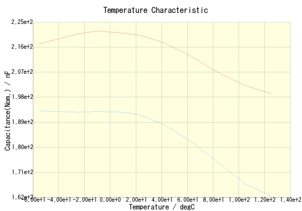
C1608X7R1C224K080AC(DC Bias = 0V) C1608X7R1C224K080AC(DC Bias = 8V)
