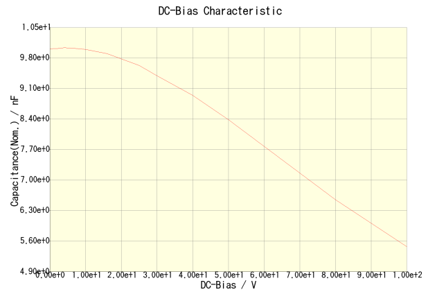
C2012X7R2A103K085AA
