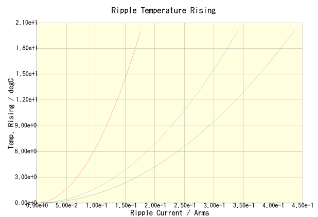
C2012X7R2A103K085AA(100kHz) C2012X7R2A103K085AA(500kHz) C2012X7R2A103K085AA(1MHz)
