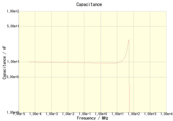
C2012X7R2A103K085AA
