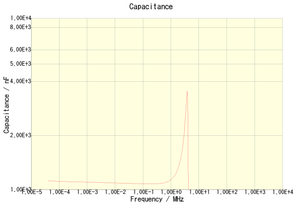
C3216X7R2A105K160AA
