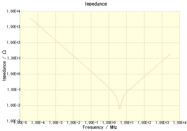
C3216X7R2A105K160AA
