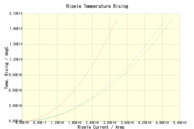
C2012X5R1E106K125AB(100kHz)
