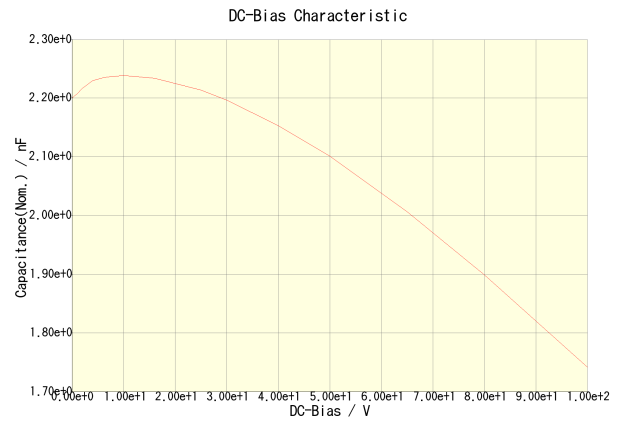
C1608X7R2A222K080AA
