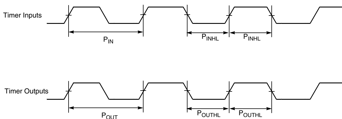
Figure 34. Timer Timing
