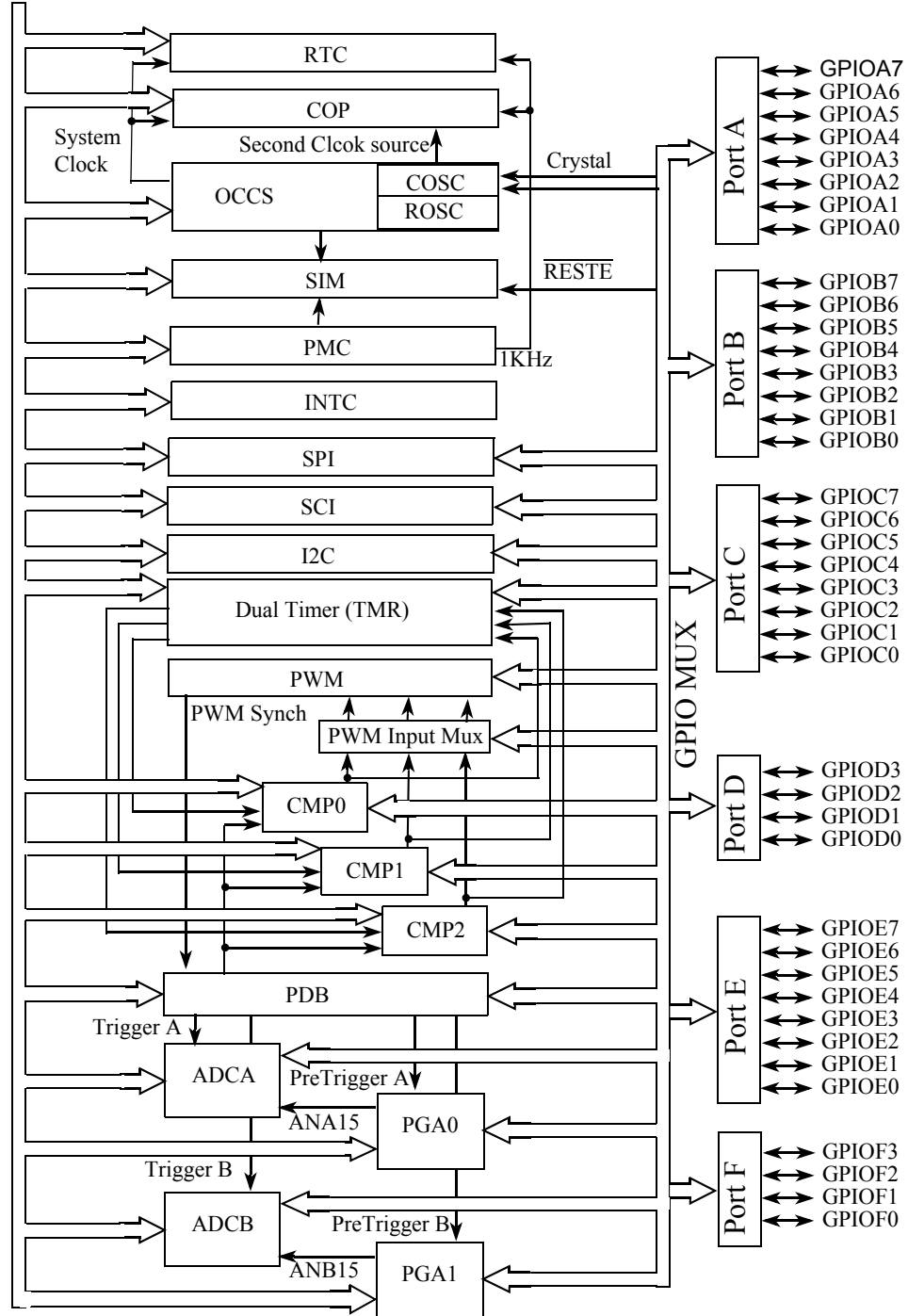
Figure 3. Peripheral Subsystem
