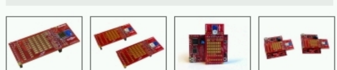
RF BoosterPack with the CC110L module from Anaren
