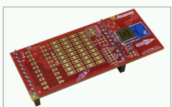
RF BoosterPack with the CC110L module from Anaren
