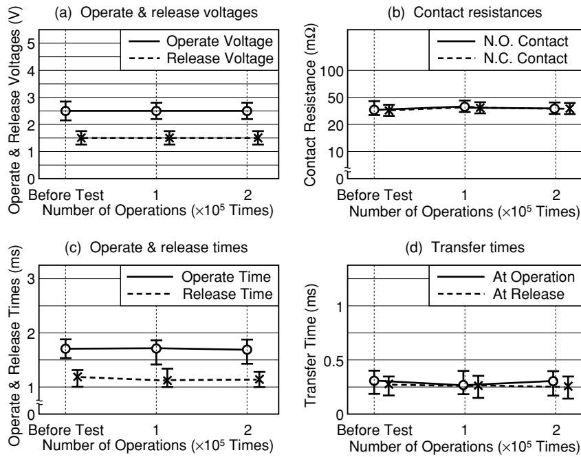
Figure 5.18 Resistive Load Test G
