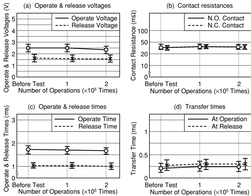
Figure 5.17 Resistive Load Test F
