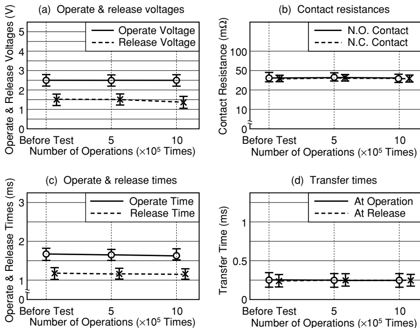
Figure 5.15 Resistive Load Test E
