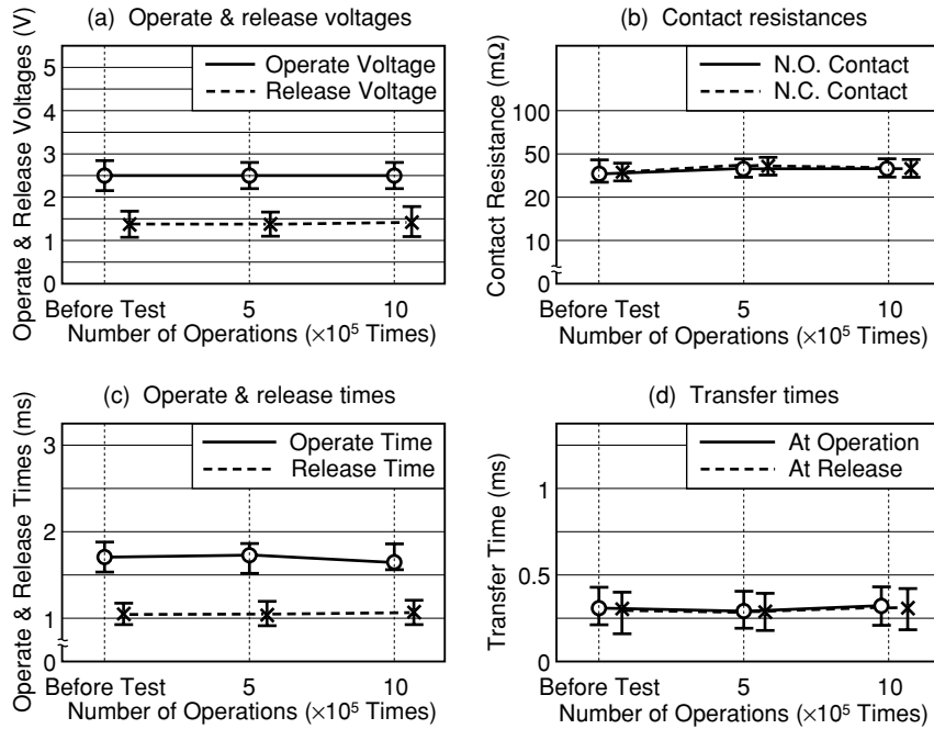
Figure 5.16 Inductive Load Test
