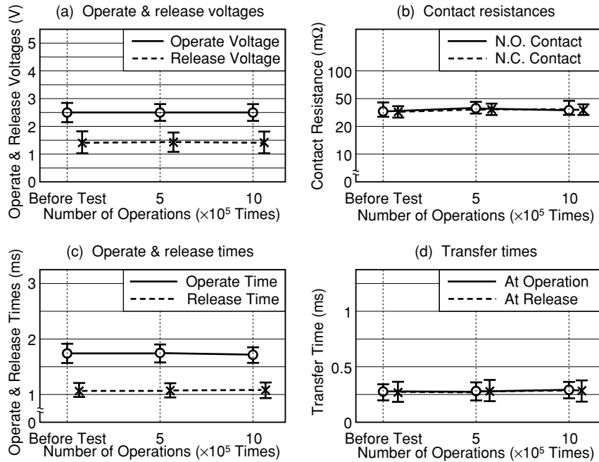
Figure 5.14 Resistive Load Test D
