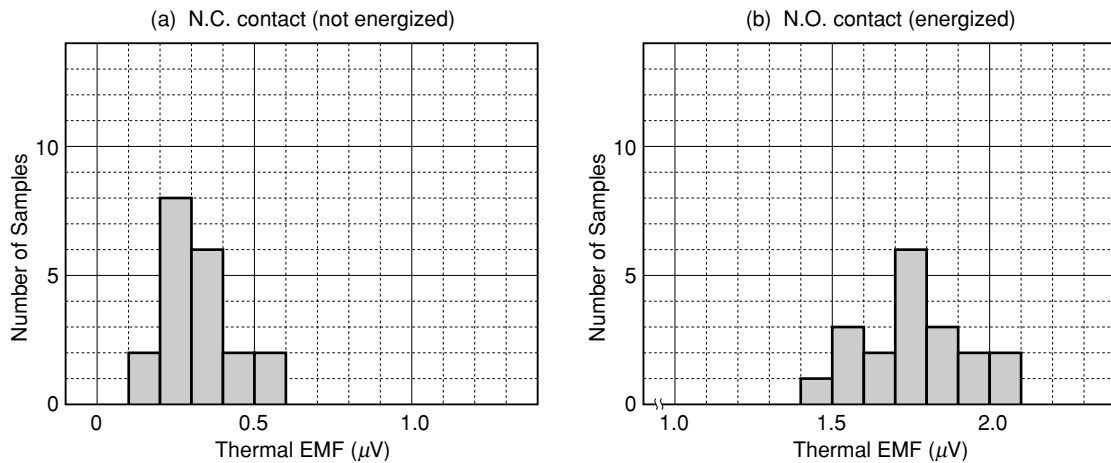
Figure 4.7 Thermal EMF
