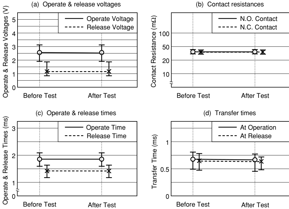
Figure 5.2 (1) Low-temperature Test
