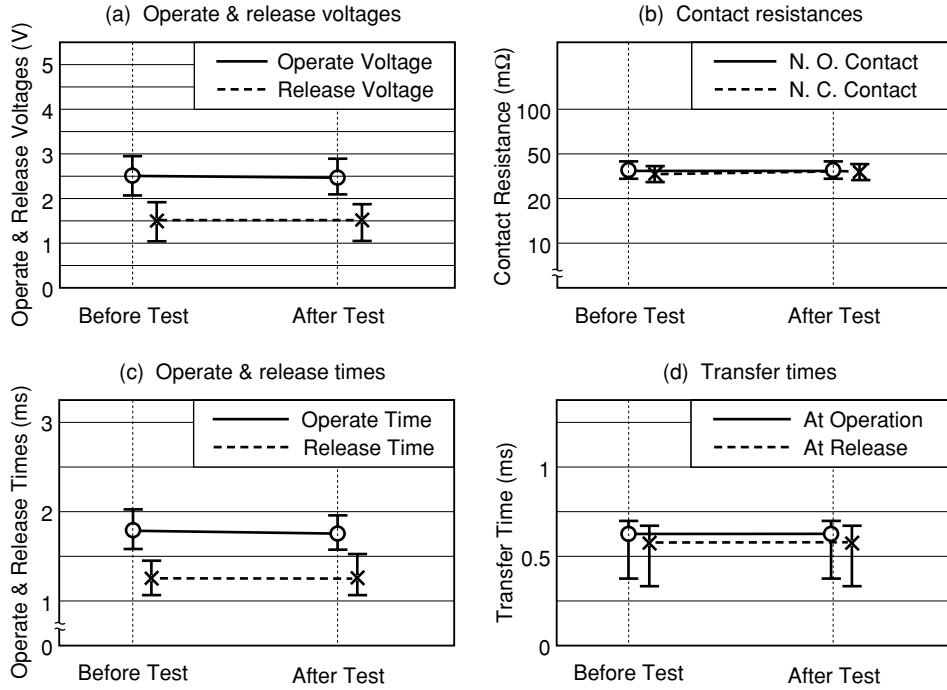
Figure 5.8 (1) Terminal Strength
