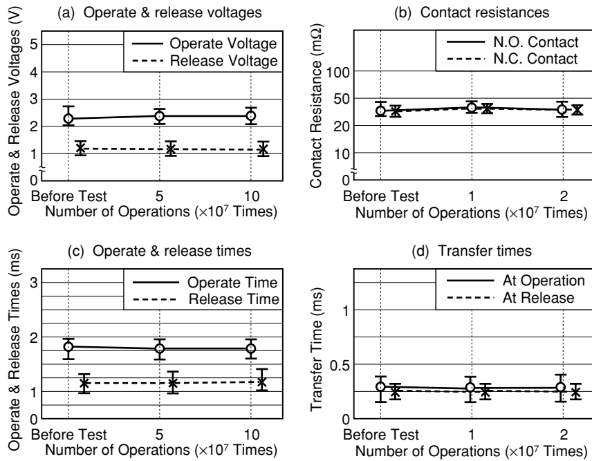
Figure 5.10 Non-load Test B
