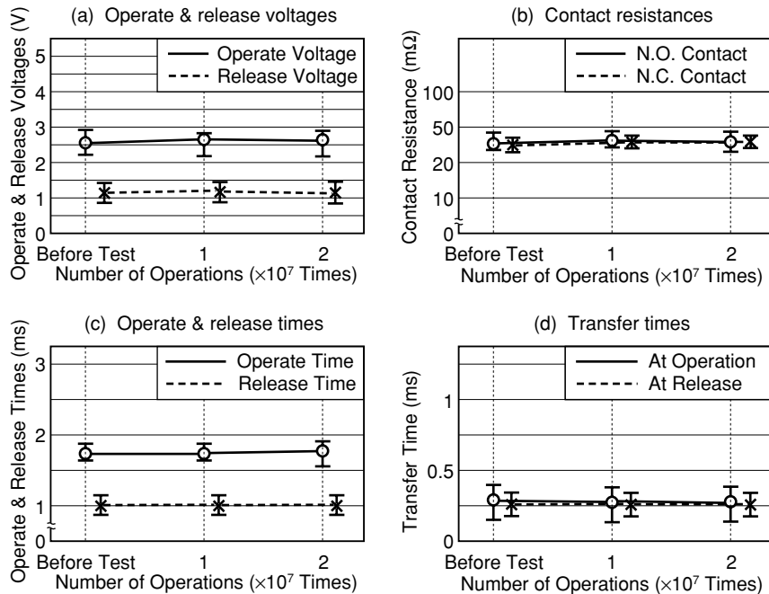
Figure 5.11 Resistive Load Test A
