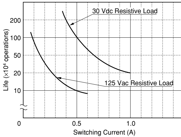
Figure 3.2 Life Curve
