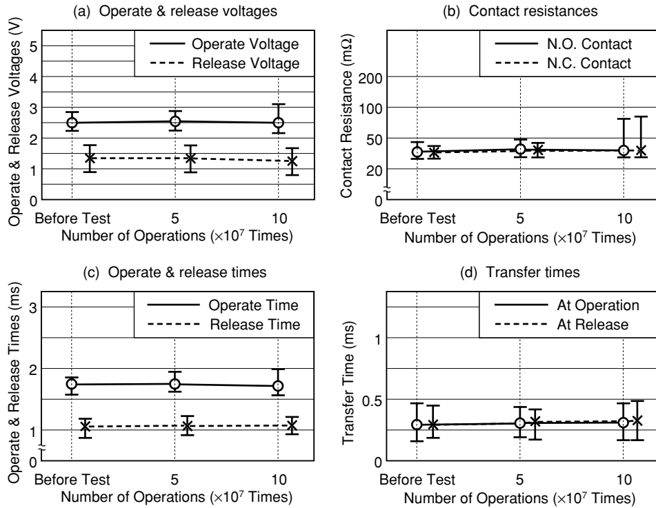
Figure 5.9 Non-load Test A
