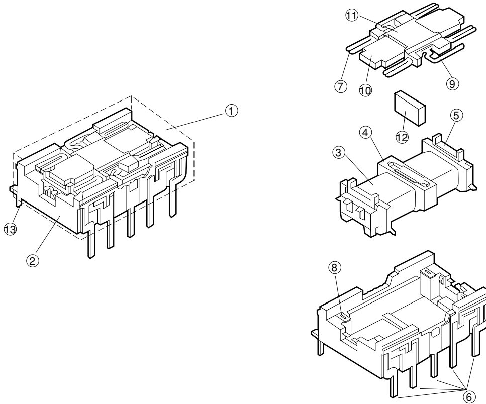
Figure 2.1 Structure of the EA2 Series Relay
