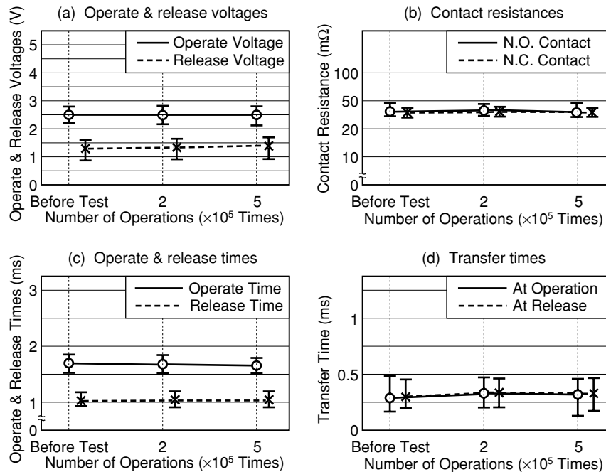
Figure 5.13 Resistive Load Test C
