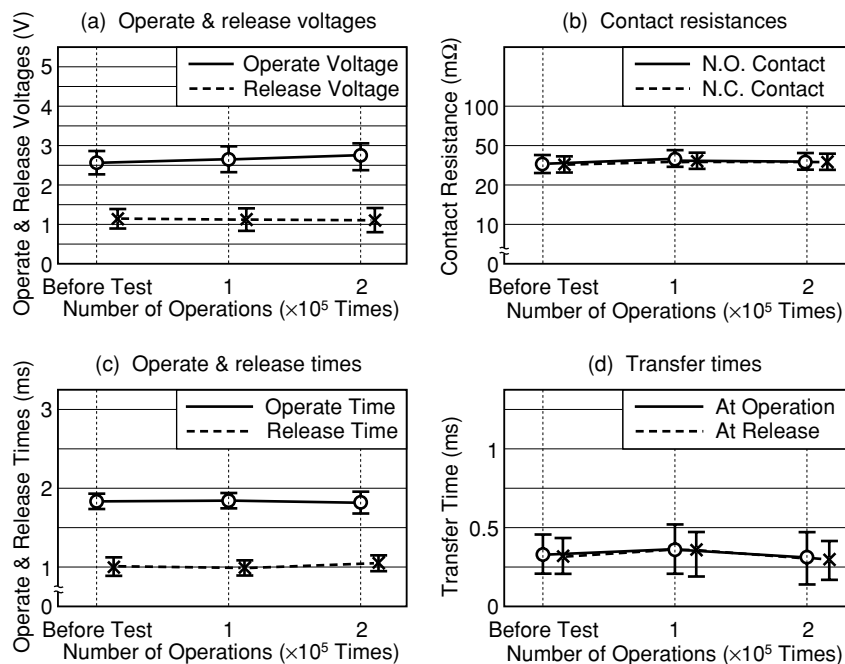
Figure 5.19 Resistive Load Test H
