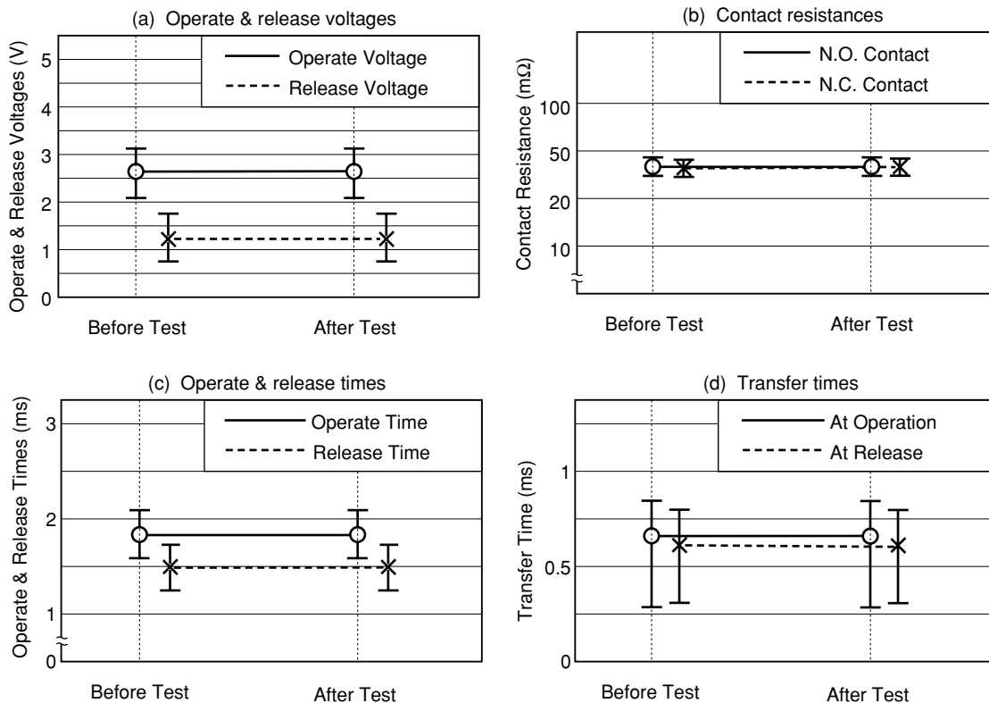
Figure 5.1 (1) High-temperature Test
