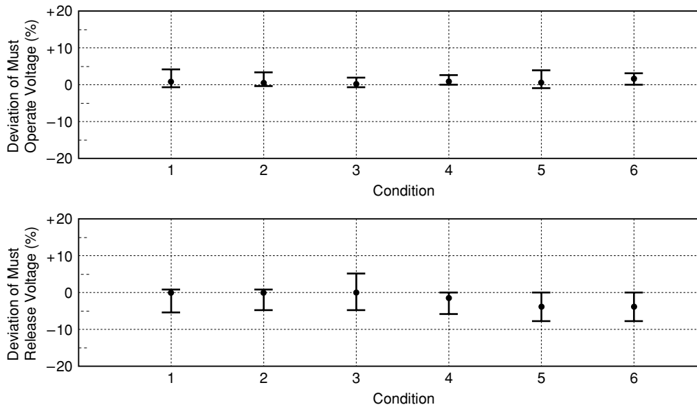
Figure 3.8 Magnetic Interference
