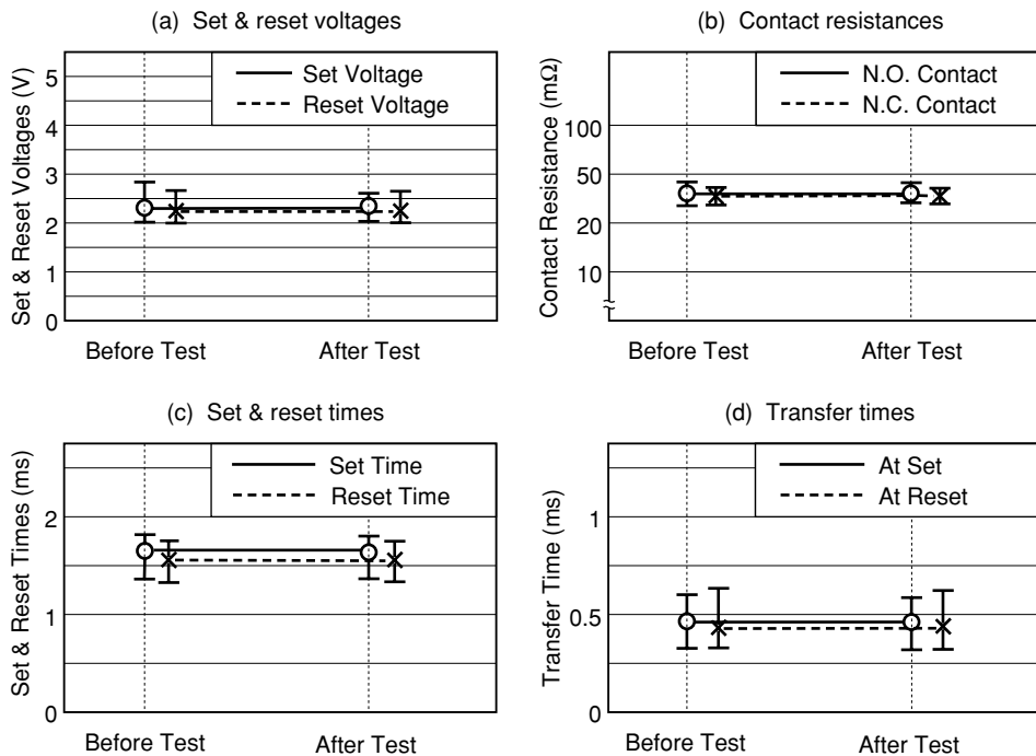
Figure 5.8 (2) Terminal Strength
