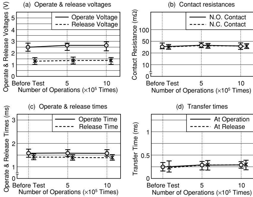
Figure 5.12 Resistive Load Test B
