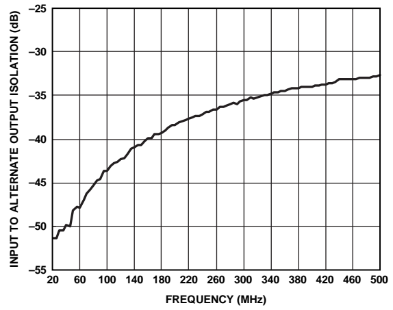
Figure 12. Device-to-Device Isolation vs. Frequency
