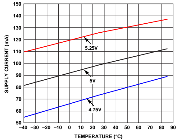
Figure 14. Supply Current vs. Temperature and Supply Voltage
