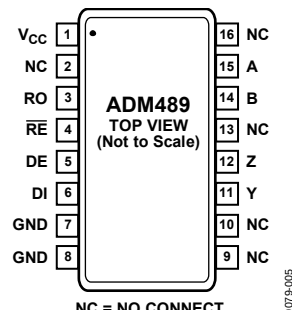
Figure 5. ADM489 16-Lead TSSOP Pin Configuration
