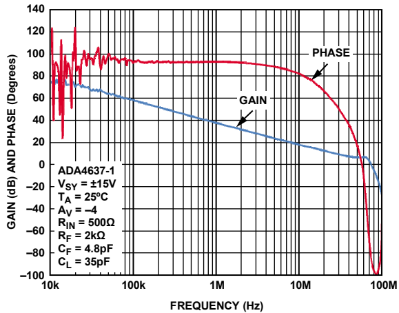
Figure 36. Open-Loop Gain and Phase vs. Frequency
