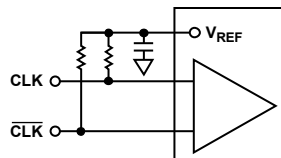
Figure 32. Use of the V_{REF} to Provide Low Impedance Termination into V_S/2
