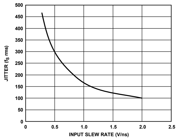
Figure 11. Additive Broadband Jitter vs. Input Slew Rate
