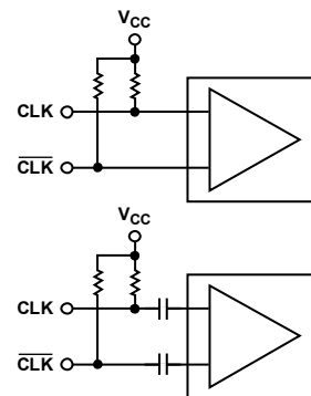
Figure 29. Typical AC-Coupled or DC-Coupled CML Configurations (see Table 8 for CML Coupling Limitations)
