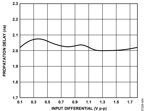
Figure 4. LVDS Propagation Delay vs. V_{ID}
