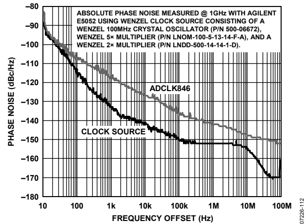
Figure 12. Absolute Phase Noise LVDS at 1000 MHz
