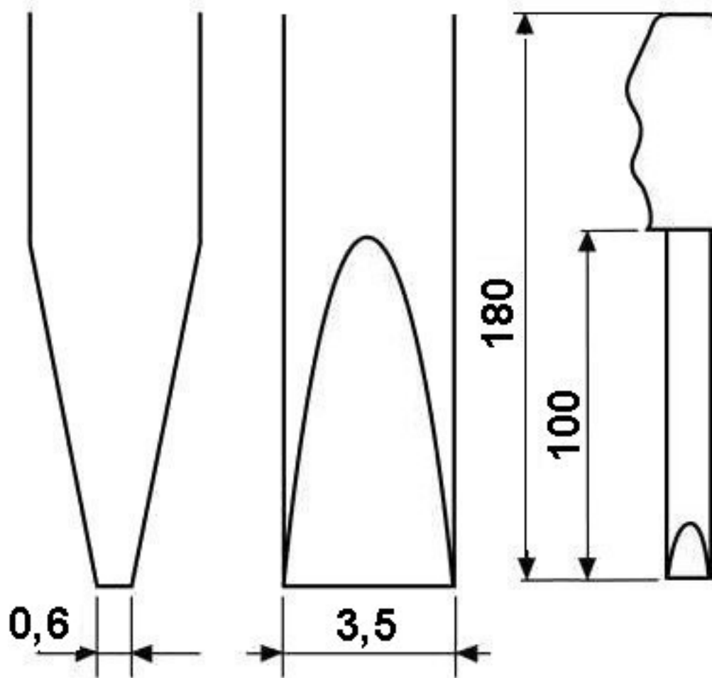
Dimensioned drawing
