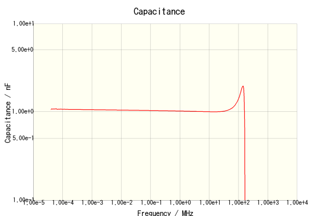
C2012X7R2A102K085AA
