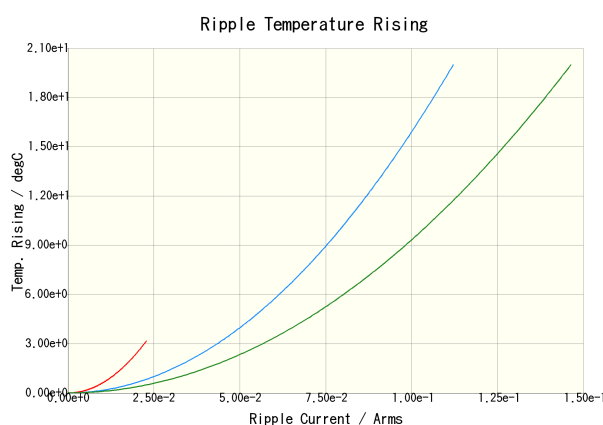
C2012X7R2A102K085AA(100kHz) C2012X7R2A102K085AA(500kHz) C2012X7R2A102K085AA(1MHz)
