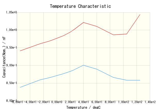
C2012X7R2A102K085AA(DC Bias = 0V) C2012X7R2A102K085AA(DC Bias = 50V)
