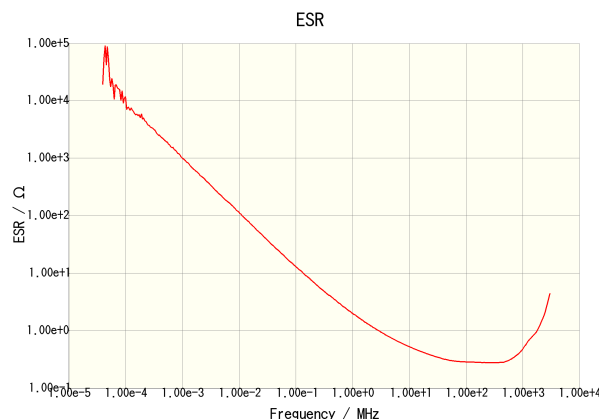
C2012X7R2A102K085AA
