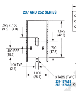
237 AND 252 SERIES Dimensions: in. (mm)
