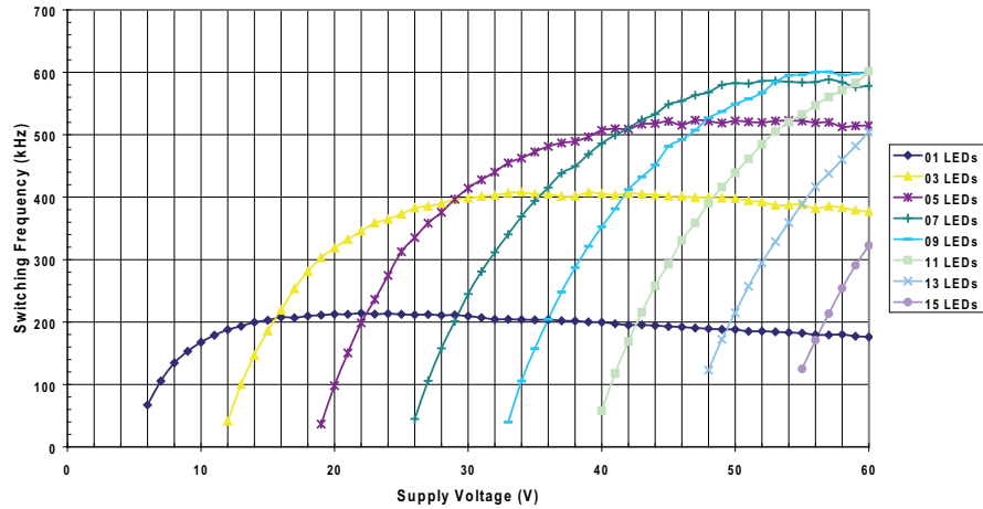
ZXLD1356 Switching Frequency L=68μH
