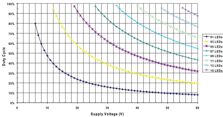
ZXLD1356 Duty Cycle L=68μH
