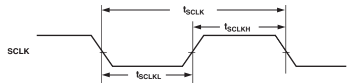
Figure 44. SCLK Timing Requirements
