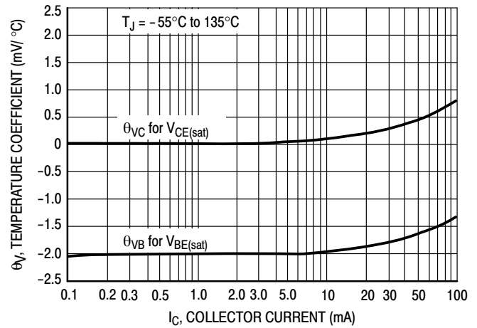
Figure 7. Temperature Coefficients
