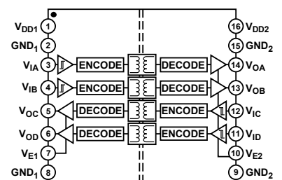
Figure 3. ADuM1402
