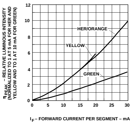
Figure 10. Relative Luminous Intensity vs. DC Forward Current.
