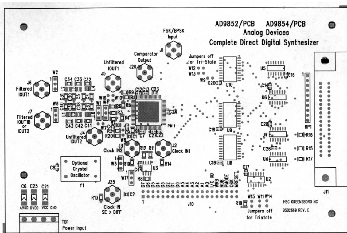
Figure 63. Assembly Drawing
