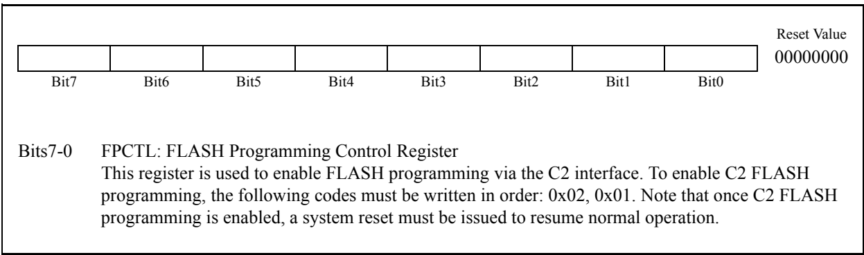
Figure 17.4. FPCTL: C2 FLASH Programming Control Register
