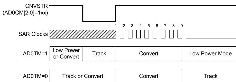
Figure 5.4 8-Bit ADC Track and Conversion Example Timing
