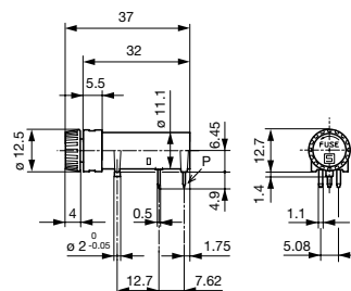
Variant Fingergrasp 3101.0055
