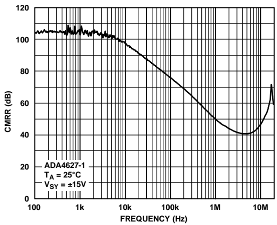
Figure 6. CMRR vs. Frequency
