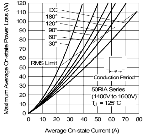
Fig. 10 - On-state Power Loss Characteristics
