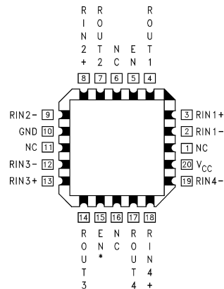
LCC Package
