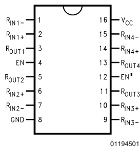
Dual-In-Line
